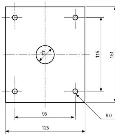
Frontansicht - Montageplatte / Front view - mounting plate
